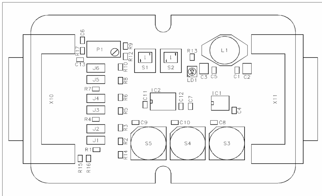
Figure 9: Component side
