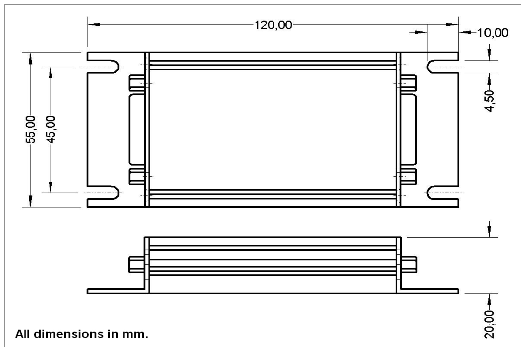
Figure 10: Dimensions
