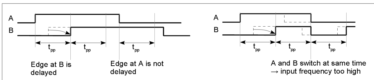
Figure 6: Minimum Edge Distance
